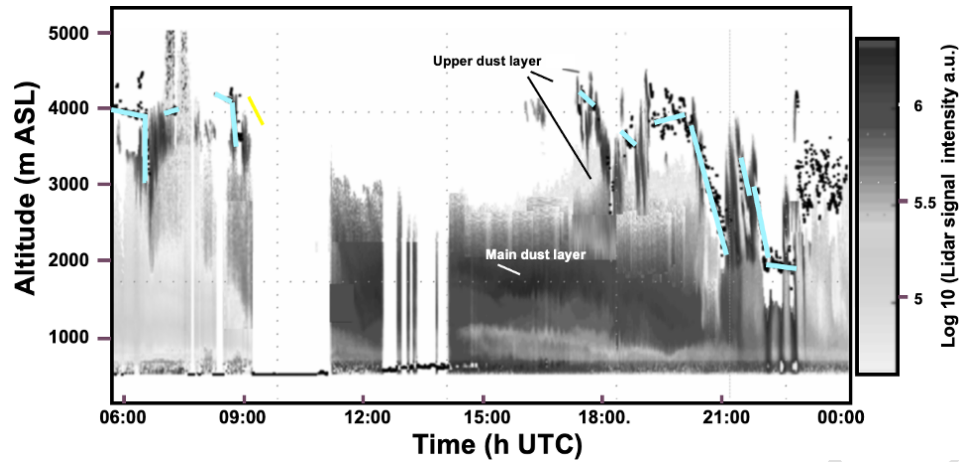
Figure 5. Ceilometer profile for 6 February (MeteoSwiss). The small black dots and blue lines above the reflections indicate the meteorological cloud base. The white strips are gaps due to ground fog.
