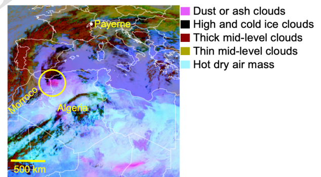
Figure 3. Satellite RGB image (5 February TS7 2021, 22:00 UTC) from the SEVIRI dust product. The dust plume transported to central Europe is seen east of the Moroccan–Algerian border (center of the yellow circle).
