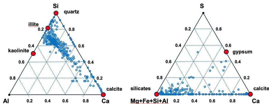
Figure 11. Ternary diagrams: (a) (\text{Mg} + \text{Fe} + \text{Si} + \text{K} - \text{Al} - \text{Ca}) , (b) (\text{Mg} + \text{Fe} + \text{Si} + \text{K} - \text{S} - \text{Ca}) .
