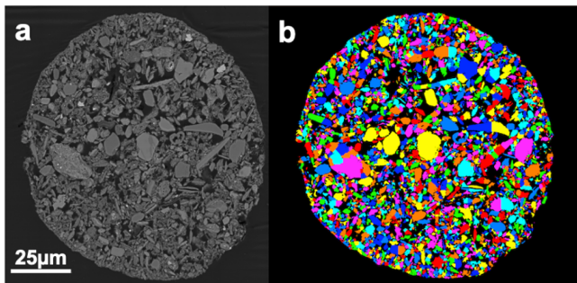
Figure 9. (a) BSE image of a polished section through an iberulite and (b) the corresponding segmentation obtained from Aviso (CE10). The different colors are used to better distinguish individual particles but do not represent any specific elemental composition.
