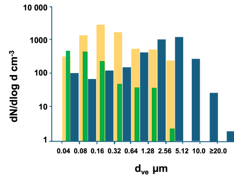
Figure 10. Jungfraujoch PSD measured in April 2004, when JFJ was above the PBL and cloud-free, and there was no SDE (green bars); during the SDE of 6 February at 12:00 UTC (yellow bars, shifted one bin to the left relative to the original data; see text); and for an iberulite sample collected in Saint-Légier (blue bars).
