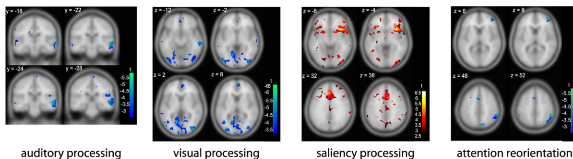
Fig. S4. (Top) Single-subject (three sessions recorded inside the scanner and one session outside) and (Middle) group-level template maps of the four dominant EEG microstates. (Bottom) fMRI activation maps revealed by GLM analysis of the microstate occurrences after convolution with the hemodynamic response (1). (Reprinted from ref. 1, with permission from Elsevier.)
