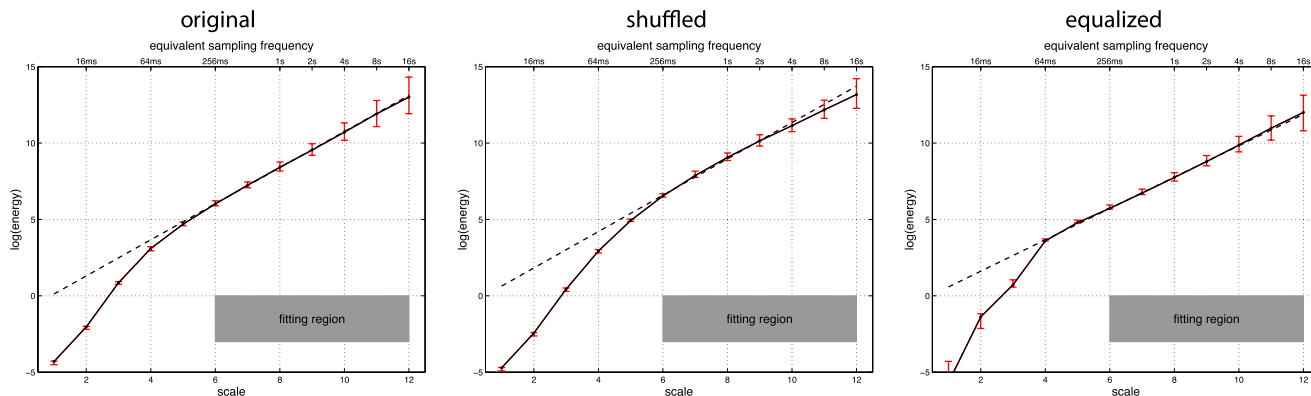
Fig. S1. The log-scaling diagrams (pooled over all subjects, sessions, and possible bipartitions) of the various microstate sequences show the energy of the wavelet coefficients as a functions of scale j , which corresponds to \log_2(2^j S(d_X, j, 2)) . The equivalent sampling frequency is indicated on the upper horizontal axis. We determined the fitting region as the part of the log-scaling diagram the shows a power law, i.e., between 256 ms and 16 s. The fitting of the power law is plotted as a dashed line. The error bars indicate the 10% and 90% percentiles.
