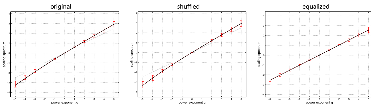
Fig. S3. The scaling spectra (pooled over all subjects, sessions, and possible bipartitions) of the various microstate sequences reveal the fractal signature of the microstate sequences. A linear trend reflects monofractality, whereas multifractality is characterized by a departure from linearity; i.e., the Hurst exponent H corresponds to the slope of the scaling spectrum and higher-degree cumulants c_2 and c_3 capture multifractal deviations. The dotted line indicates the scaling spectrum of white noise ( H = 0.5 ). The error bars indicate the 10% and 90% percentiles.
