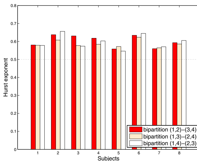
Fig. S2. Hurst exponent obtained using wavelet fractal analysis for the original microstate sequences and different choices of the bipartitions, for all subjects.
