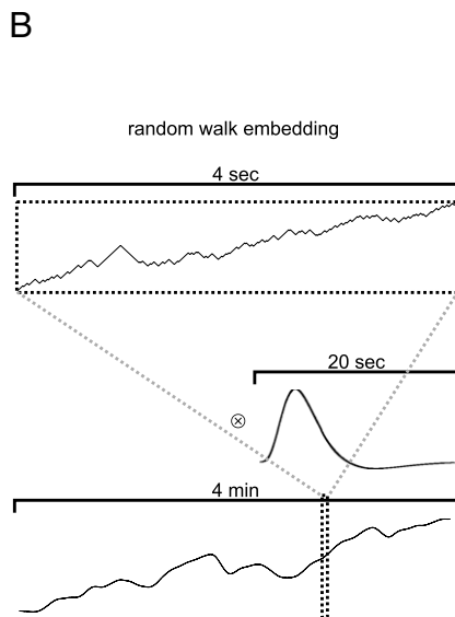
Fig. 1. (A) Illustration of the link between EEG microstates and their manifestation at the fMRI level. Our recent work (25) showed that after convolution of the EEG microstate sequences with the hemodynamic response function, which introduces a strong temporal smoothing, the resulting signals correlate significantly with large-scale RSNs. (B) To investigate the intriguing link between microstate sequences at the EEG and fMRI level, we study the fractal properties of their random walk embedding. Scale-free dynamics or statistical self-similarity is reflected by the same behavior of the random walk at various timescales.
