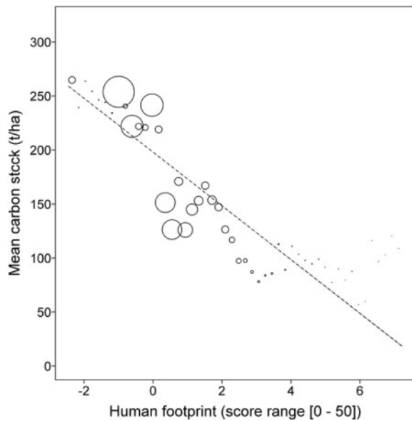
Fig. 5 Relationship between the carbon stock and human footprint. Legend: The area of the circle corresponds to the number of data points. All points are binned data points for a fraction on the x and y axis with the mean per fraction. The point is bigger when more data points fall into this fraction. The dashed line depicts the fitted model
