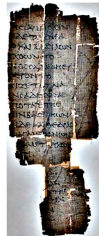
retinex
