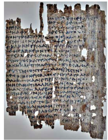
retinex
