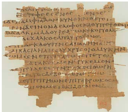
locallapfilt
