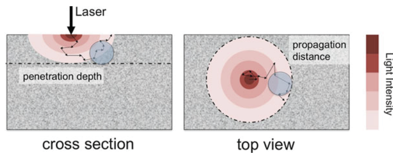
Fig. 4 Diffuse scattering of light in reflection. The incident wave is dispersed and scattered along a path of a certain contour length. The scattered wave leaves the sample at a distance \rho_{xy} \leq 3l_t . The propagating waves reach a typical depth z of about half this distance [35, 36]. If only a section of the light path crosses a region of interest ( blue shaded circle ), the effective path length inside this region needs to be considered only. Modeling the latter is difficult if the sample is accessed only from a single perspective. The problem can however be overcome using optical tomography based on a numerical analysis of the signal obtained from a number of different source/detector pairs placed around the object [24].
