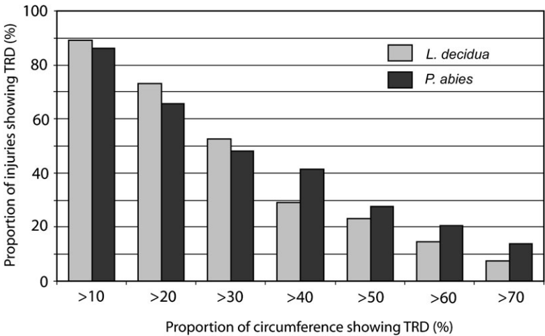
Figure 4. Radial spread of TRDs in that portion of the tree ring remaining vital in the first year following wounding.
