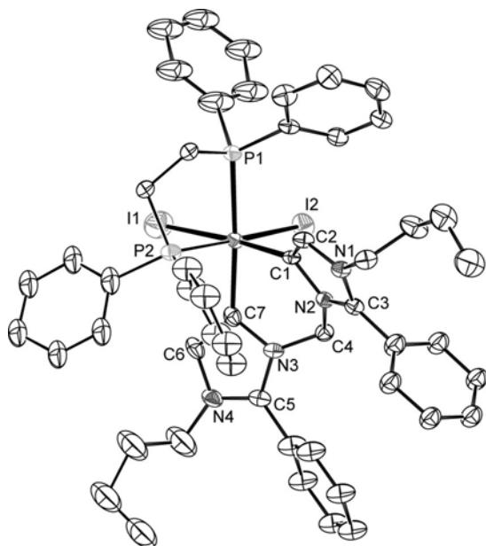
Figure 3. ORTEP representation of complex 7 (30% probability level, hydrogen atoms, the cocrystallized ether molecules, and the \text{I}^- anion omitted for clarity; only one of the two disordered positions of the \text{CH}_2\text{CH}_2\text{PPh}_2 moiety of the dppe ligand is shown). Selected bond lengths ( \text{\AA} ): Rh1–C1 2.031(9), Rh1–C7 2.050(10), Rh1–I1 2.6359(12), Rh1–I2 2.7209(10), Rh1–P1 2.357(2), Rh1–P2 2.237(13), C1–C2 1.370(12), C6–C7 1.352(13). Selected bond angles (deg): C1–Rh1–C7 88.3(4), C1–Rh1–I1 175.9(2), C1–Rh1–I2 92.4(2), C1–Rh1–P1 92.6(2), C1–Rh1–P2 94.9(3), C7–Rh1–P1 176.4(2), C7–Rh1–P2 90.1(4), P1–Rh1–P2 86.7(3), I1–Rh1–I2 89.85(4).
