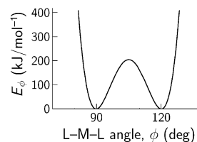
Figure 2. Double-well function with minima at 90^\circ and 120^\circ . With h = 500 , it was possible to approximate the curvature in the vicinity of the minima comparable to that obtained with normal harmonic functions for L-M-L angle bending.
