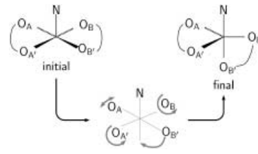
Figure 4. A sketch of the SQP \rightleftharpoons TBP ax interconversion path. It shows that both acac rings undergo specific concerted angular-distortions at the Ni atom, and maintain approximate bilateral symmetry if the chelate rings are neglected (see text for further description of the interconversion mechanism).
