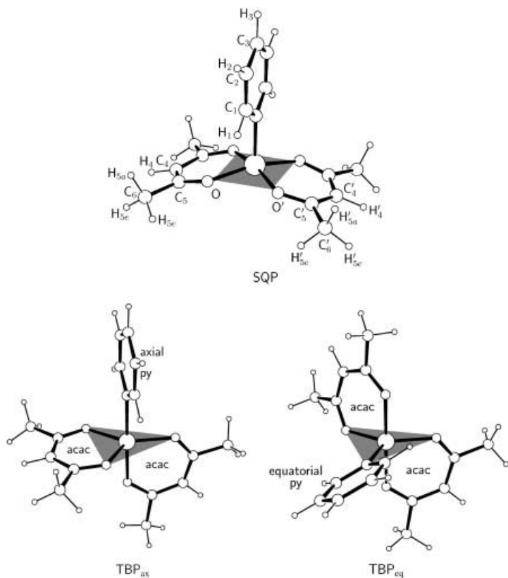
Figure 1. Three polytopal forms of [\text{Ni}(\text{acac})_2(\text{py})] : square pyramid (SQP) with the atom numbering scheme, trigonal bipyramid with axial unidentate py ( \text{TBP}_{\text{ax}} ), and trigonal bipyramid with equatorial unidentate py ( \text{TBP}_{\text{eq}} ). The structures fully depict optimized geometries by the DFT method.
